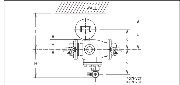
Horizontal Trim, Variable Pressure - Top View
